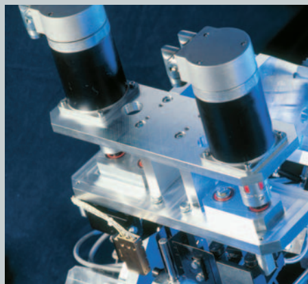
Cello tube forming unit
