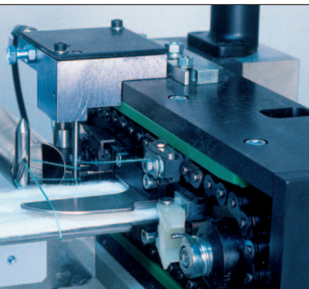
Knotter
