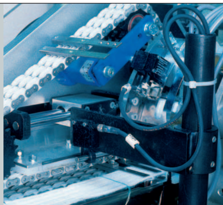
Fleece transport
