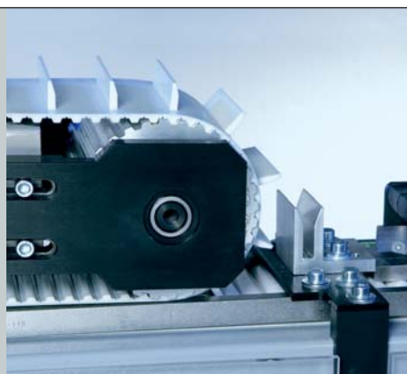
Outer tube conveyer
