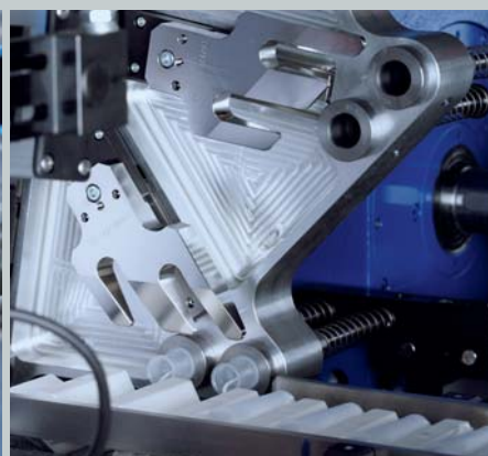
Transport drum
